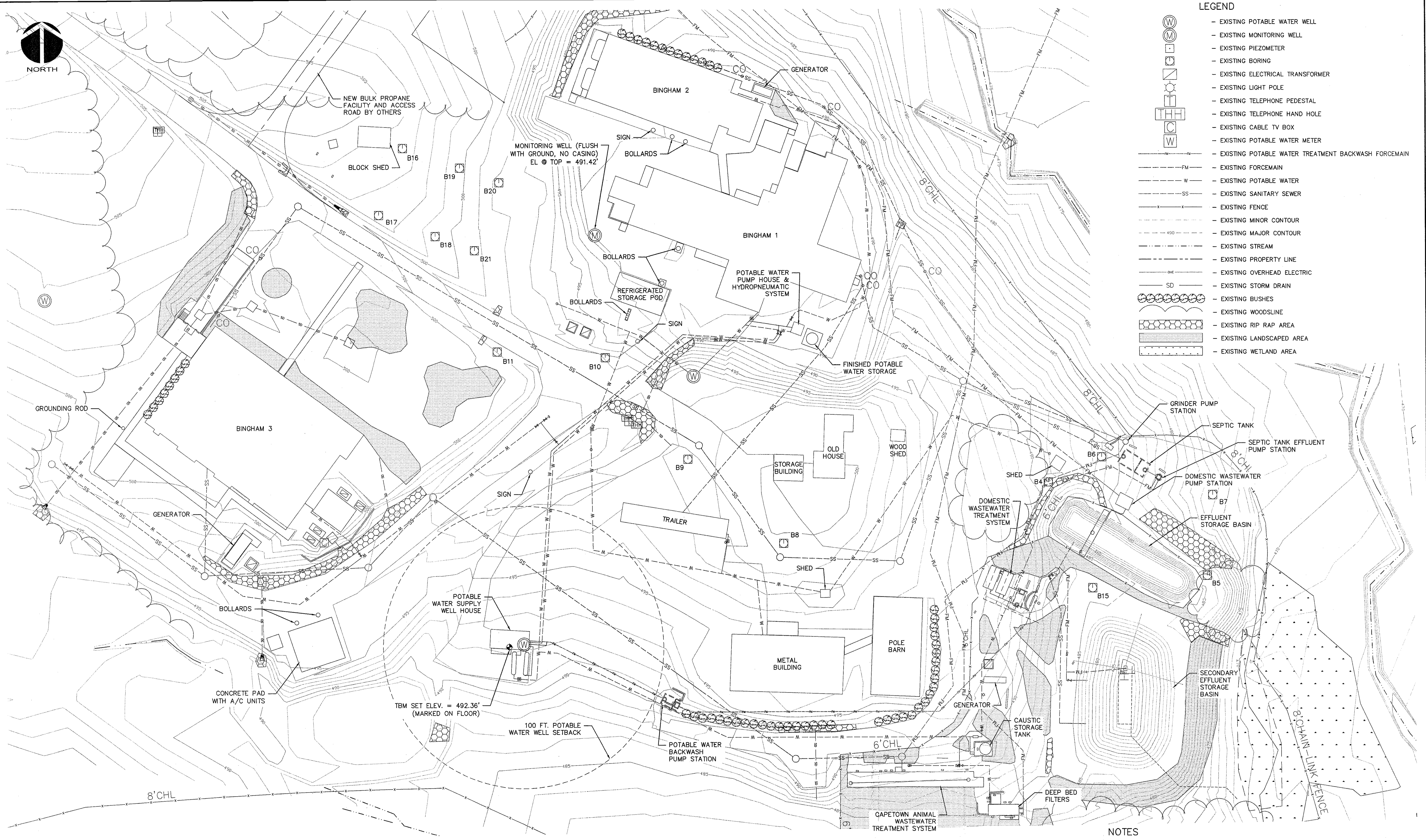
EXISTING ENLARGED SITE PLAN SCALE: 1" = 30'
